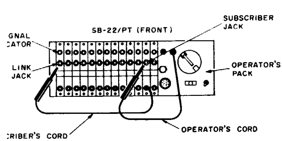
B. CORD CONNECTIONS FOR OPERATOR AND SUBSCRIBER COMMUNICATION ON RADIO LINK.
