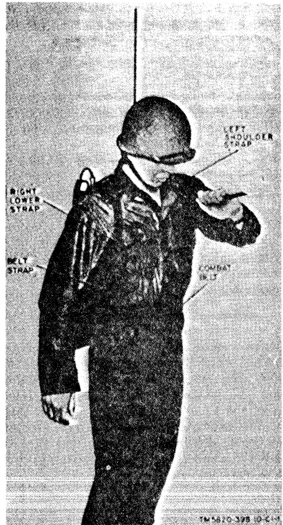
Figure 2-4. Installation AN/PRC-25 for man-pack operation.
