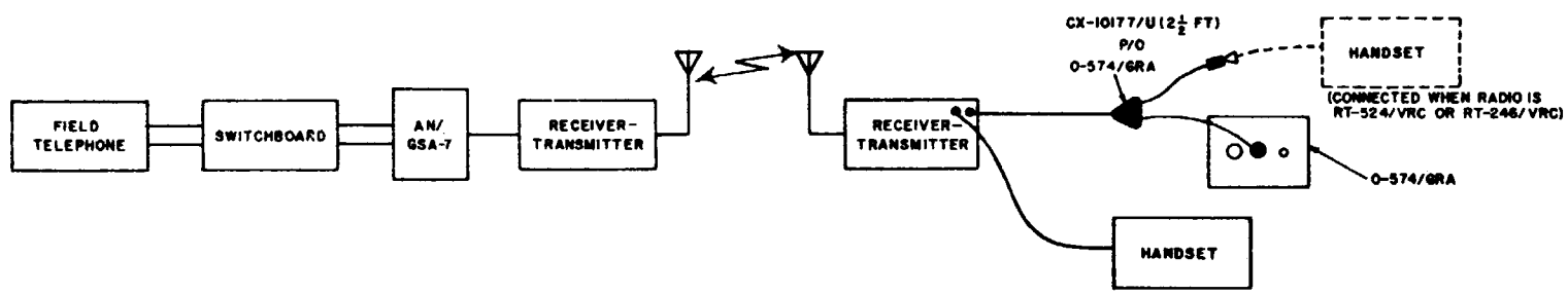
C. AN/GSA-7 AT ONE STATION, O-574/6RA AT OTHER; NO RADIO OPERATOR REQUIRED.
