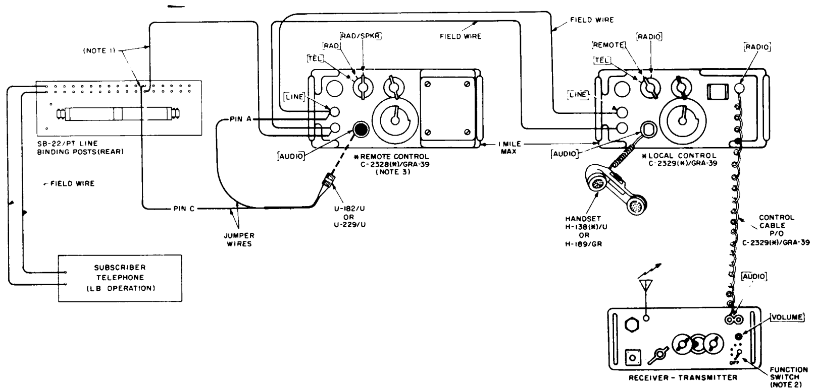
A. INTERCONNECTIONS AND SWITCH POSITIONS.
